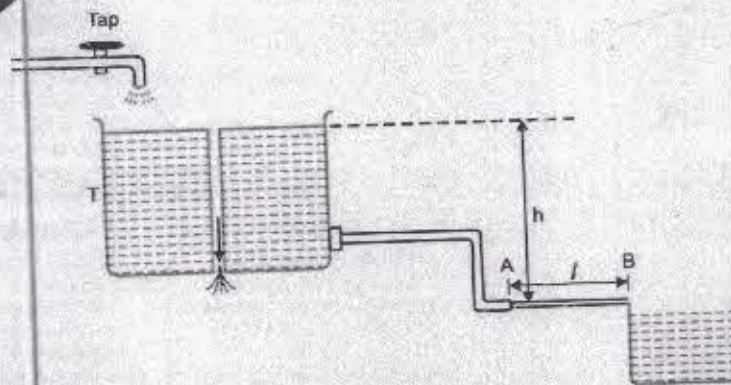
Experimental determination of viscosity of water by Poiseuille's method
